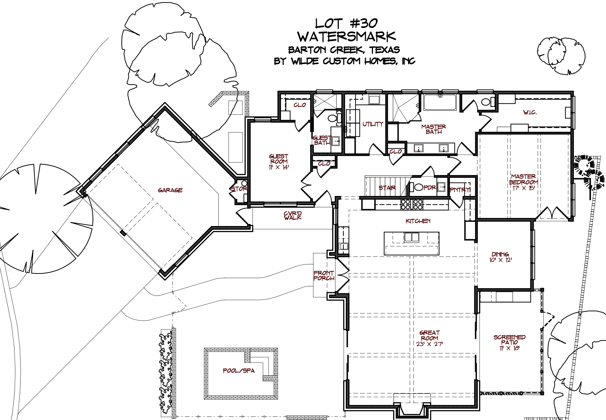
1ST FLOOR PLAN 2295 SQ FT
