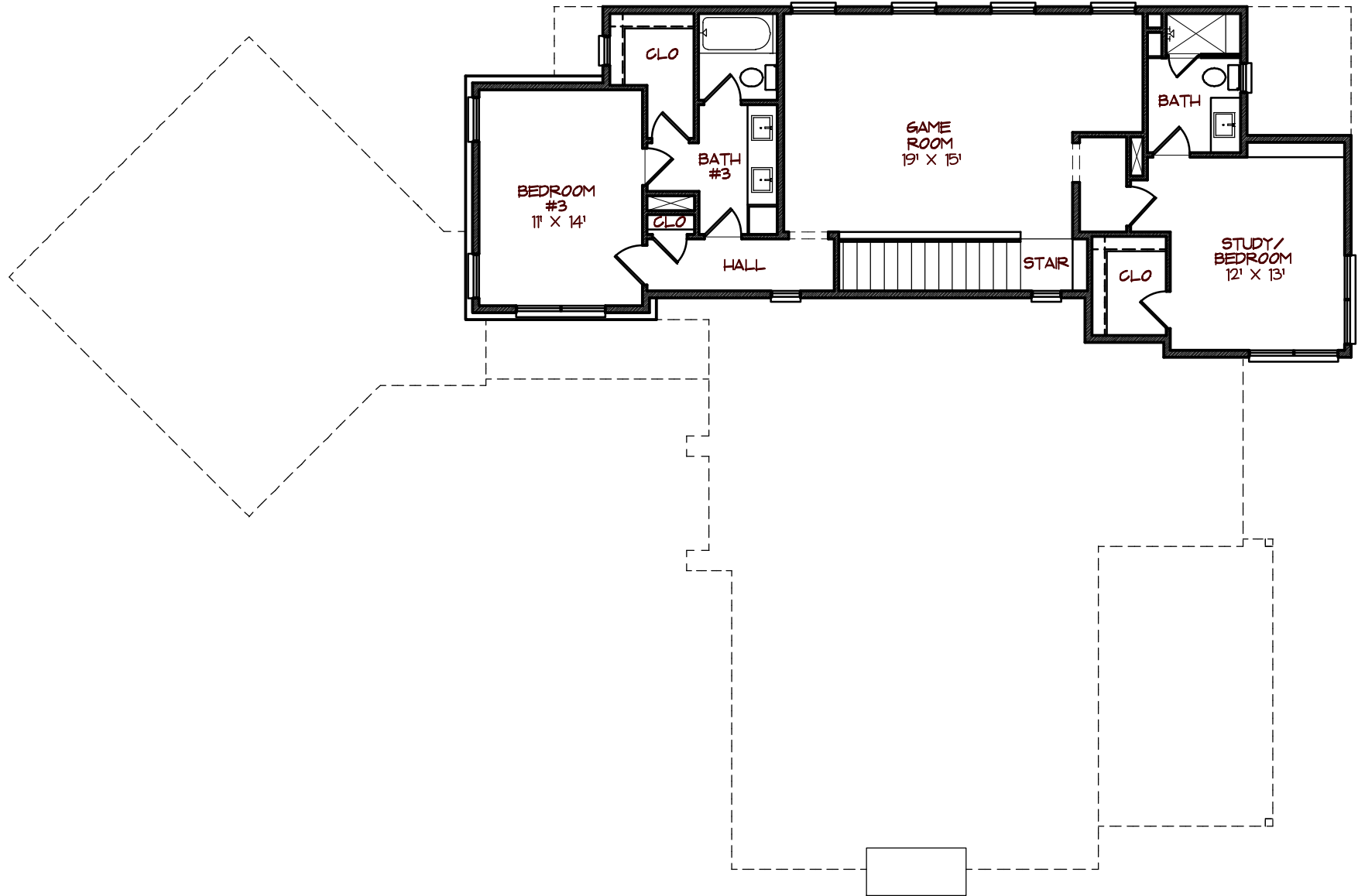
2ND FLOOR PLAN 1130 SQ FT
